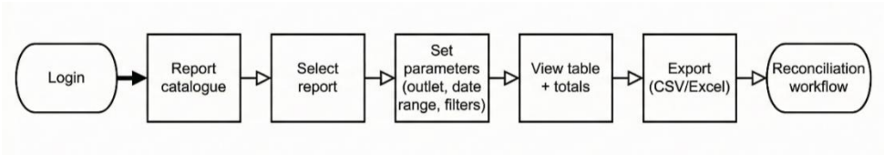
Figure 4.8: Portal navigation and report workflow (illustrative)
